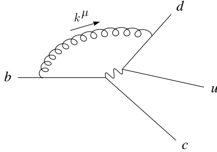
FIG. 2. The nonleptonic decay of a b quark at one loop.
